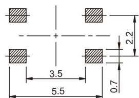
RECOMMENDED PCB LAYOUT (PCB TOLERANCE ±0.05)
