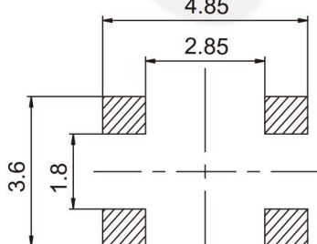
RECOMMENDED PCB LAYOUT (PCB TOLERANCE ±0.05)
