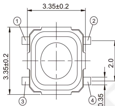
6STMS01-XXX XXX XNX A01
