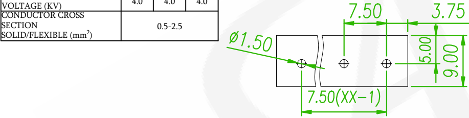
RECOMMENDED PCB LAOUT (PCB TOLERANCE ±0.05)
