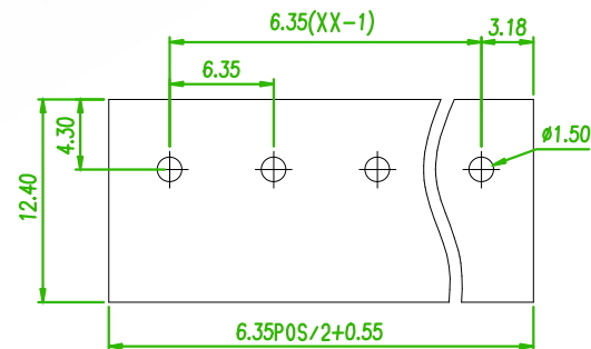
RECOMMENDED PCB LAOUT (PCB TOLERANCE ±0.05)
