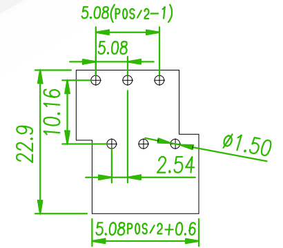
RECOMMENDED PCB LAOUT (PCB TOLERANCE ±0.05)
