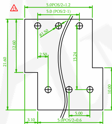
RRCOMMENDED P.C.B LAYOUT (PCB TOLERANCE±0.1)
