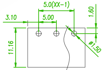
RECOMMENDED PCB LAOUT (PCB TOLERANCE ±0.05)
