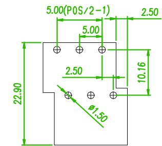
RECOMMENDED PCB LAOUT (PCB TOLERANCE ±0.05)
