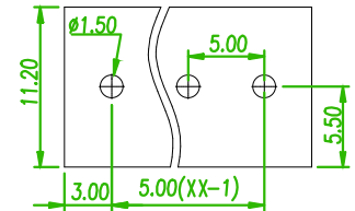
RECOMMENDED PCB LAOUT (PCB TOLERANCE ±0.05)
