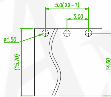
RRCOMMENDED P.C.B LAYOUT (PCB TOLERANCE±0.1)
