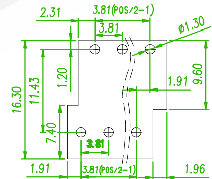
RECOMMENDED PCB LAOUT (PCB TOLERANCE ±0.05)
