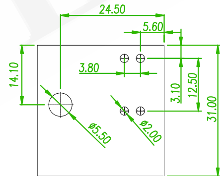
RECOMMENDED PCB LAOUT (PCB TOLERANCE ±0.05)
