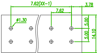
RECOMMENDED PCB LAOUT (PCB TOLERANCE ±0.05)
