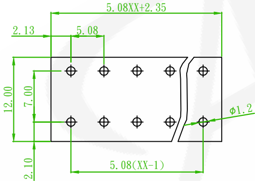
RECOMMENDED PCB LAOUT (PCB TOLERANCE ±0.05)
