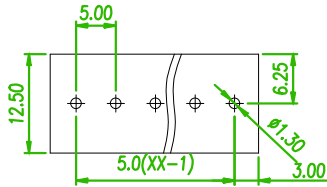
RECOMMENDED PCB LAOUT (PCB TOLERANCE ±0.05)
