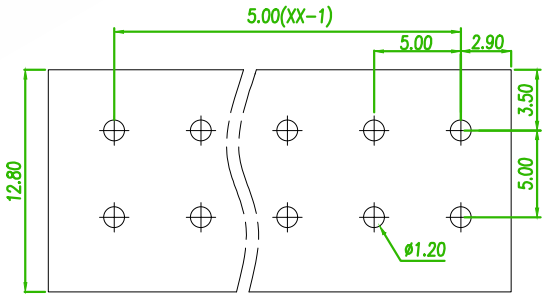
RECOMMENDED PCB LAOUT (PCB TOLERANCE ±0.05)
