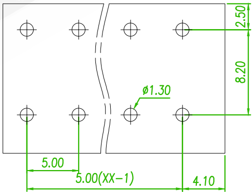
RECOMMENDED PCB LAOUT (PCB TOLERANCE ±0.05)
