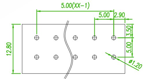
RECOMMENDED PCB LAOUT (PCB TOLERANCE ±0.05)
