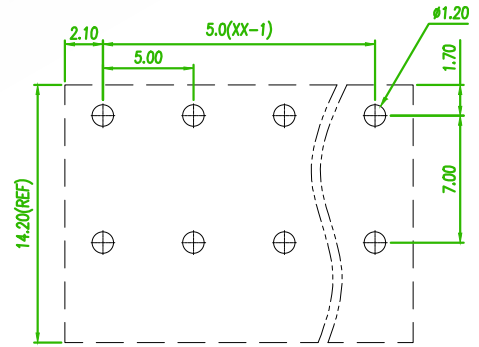
RECOMMENDED PCB LAOUT (PCB TOLERANCE ±0.05)
