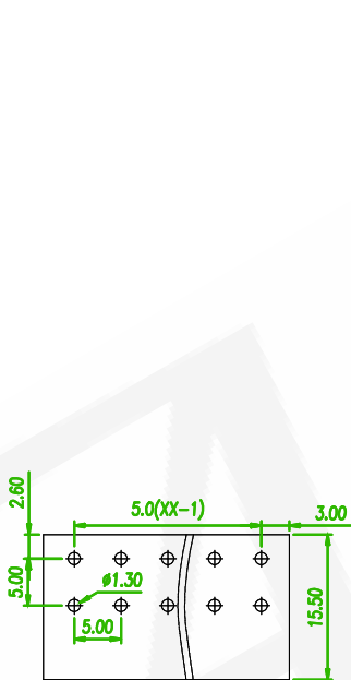
RECOMMENDED PCB LAOUT (PCB TOLERANCE ±0.05)
