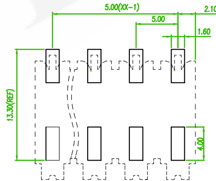
RECOMMENDED PCB LAOUT (PCB TOLERANCE ±0.05)
