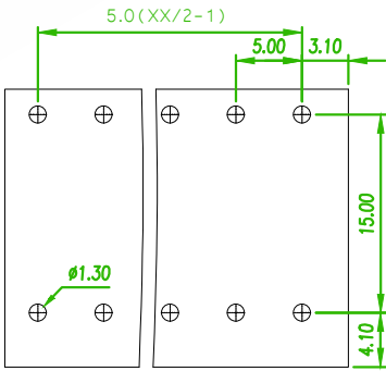
RECOMMENDED PCB LAOUT (PCB TOLERANCE ±0.05)
