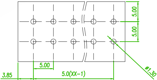
RECOMMENDED PCB LAOUT (PCB TOLERANCE ±0.05)
