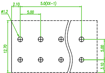
RECOMMENDED PCB LAOUT (PCB TOLERANCE ±0.05)
