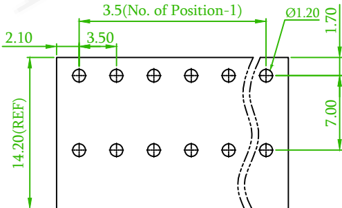
RECOMMENDED PCB LAOUT (PCB TOLERANCE ±0.05)
