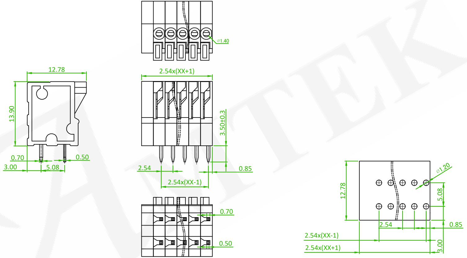
RECOMMENDED PCB LAOUT (PCB TOLERANCE ±0.05)
