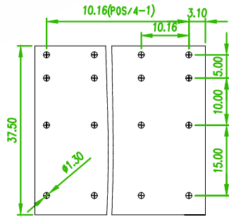
RECOMMENDED PCB LAOUT (PCB TOLERANCE ±0.05)
