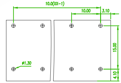
RECOMMENDED PCB LAOUT (PCB TOLERANCE ±0.05)
