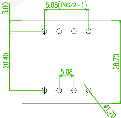
RECOMMENDED PCB LAOUT (PCB TOLERANCE ±0.05)
