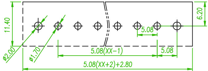
RECOMMENDED PCB LAYOUT (PCB TOLERANCE ±0.05)
