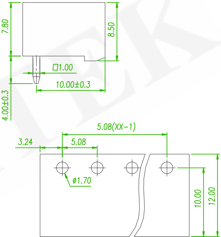
RECOMMENDED PCB LAOUT (PCB TOLERANCE ±0.05)
