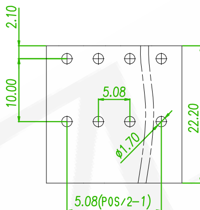
RECOMMENDED PCB LAOUT (PCB TOLERANCE ±0.05)
