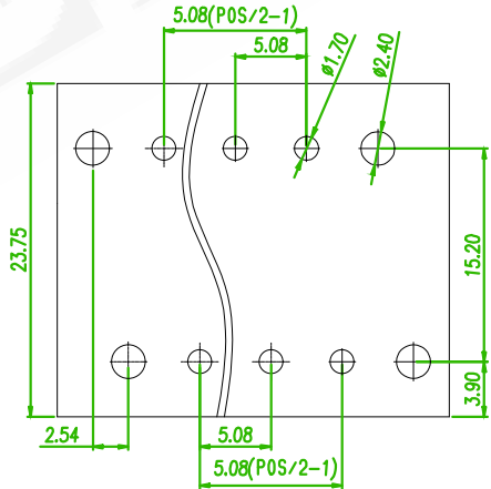
RECOMMENDED PCB LAOUT (PCB TOLERANCE ±0.05)
