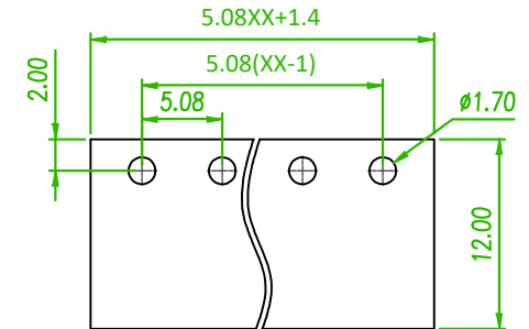
RRCOMMENDED P.C.B LAYOUT (PCB TOLERANCE±0.05)
