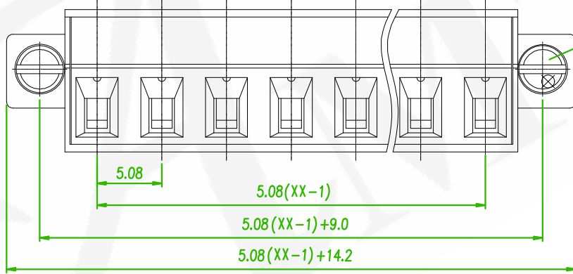
SCREW 2
