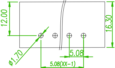
RECOMMENDED PCB LAOUT (PCB TOLERANCE ±0.05)
