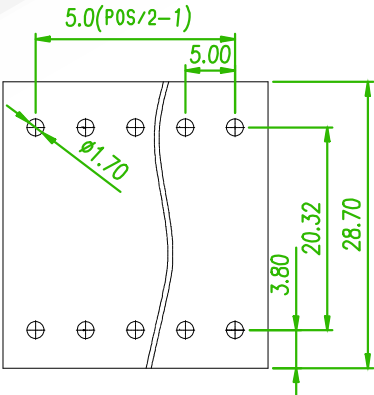
RECOMMENDED PCB LAOUT (PCB TOLERANCE ±0.05)
