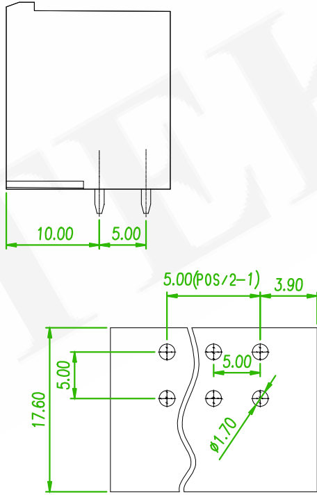
RECOMMENDED PCB LAOUT (PCB TOLERANCE ±0.05)
