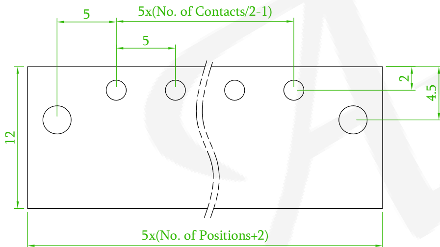
P.C.B. LAYOUT TOLERANCE: ±0.1
