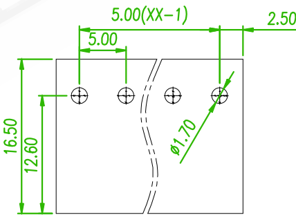
RECOMMENDED PCB LAOUT (PCB TOLERANCE ±0.05)
