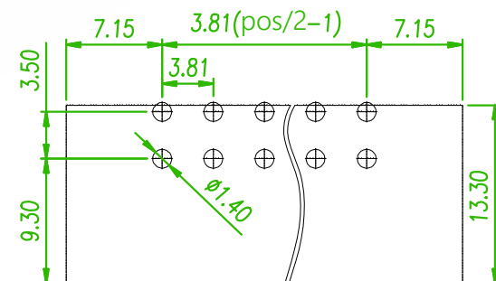
RECOMMENDED PCB LAYOUT (PCB TOLERANCE \pm 0.05 )
