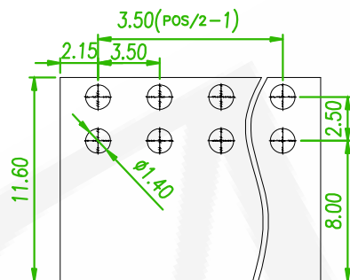
RECOMMENDED PCB LAOUT (PCB TOLERANCE \pm 0.05 )
