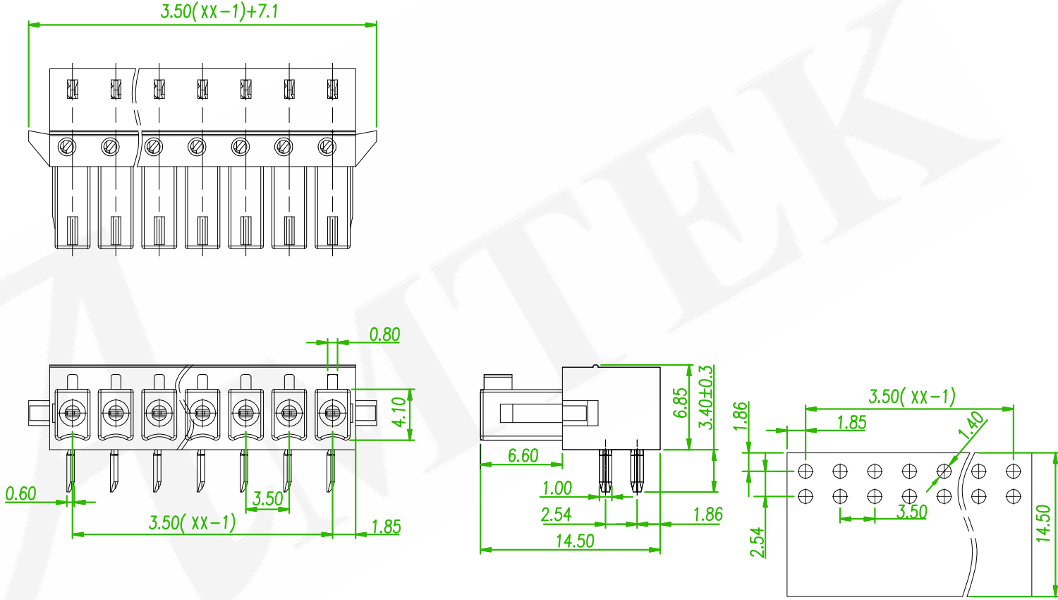
RECOMMENDED PCB LAOUT (PCB TOLERANCE ±0.05)
