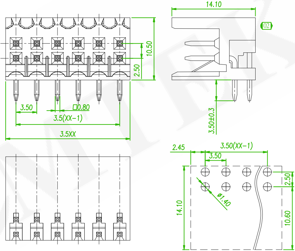
RECOMMENDED PCB LAYOUT (PCB TOLERANCE ±0.05)
