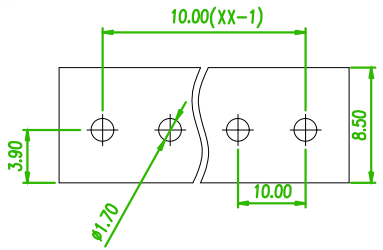
RECOMMENDED PCB LAOUT (PCB TOLERANCE ±0.05)
