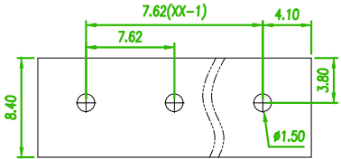
RECOMMENDED PCB LAOUT (PCB TOLERANCE ±0.05)
