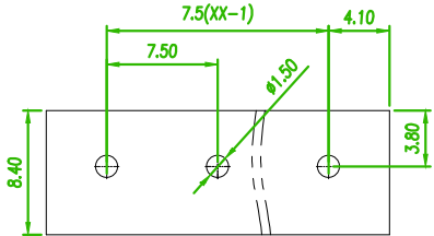
RECOMMENDED PCB LAOUT (PCB TOLERANCE ±0.05)
