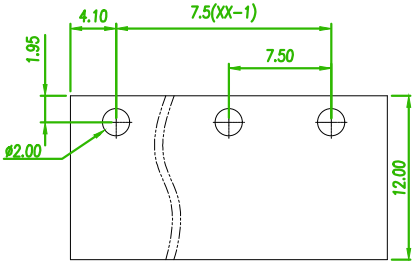
RECOMMENDED PCB LAOUT (PCB TOLERANCE ±0.05)
