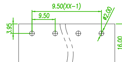
RECOMMENDED PCB LAOUT (PCB TOLERANCE ±0.05)
