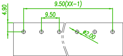
RECOMMENDED PCB LAOUT (PCB TOLERANCE ±0.05)
