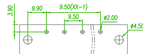
RECOMMENDED PCB LAOUT (PCB TOLERANCE ±0.05)
